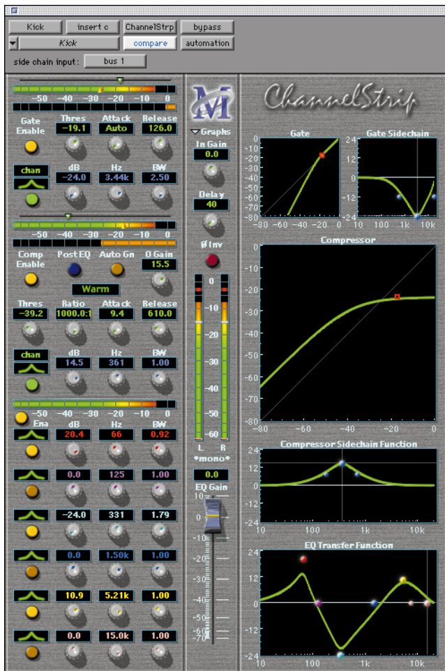
Figure 1: The ChannelStrip Plug-in Window
