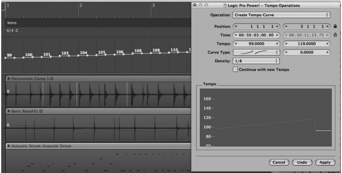
Figure 14.9 This curve was created by the Create Tempo Curve operation generating one tempo event every eighth note over the area specified by the chosen parameters.
