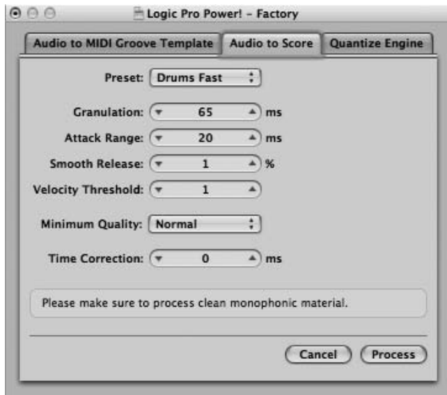
Figure 7.35 The Audio to Score dialog box.
