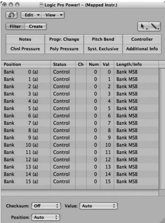
Figure 13.4 When you select a multi-instrument object, you can use the Define Custom Bank Messages command in the Environment’s local Options menu to launch this special Edit window to enter custom bank messages for your multi instrument.
