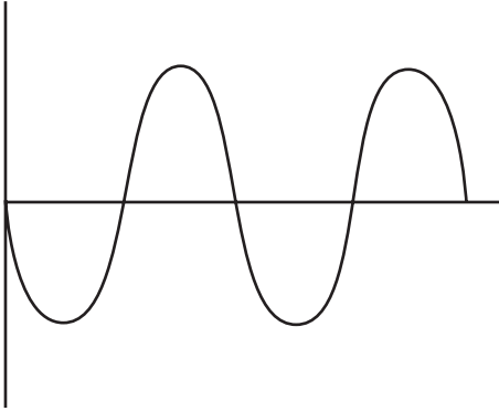
Figure 1.6 A graphical representation of a simple sound wave. This particular kind of even, smooth sound wave is known as a sine wave.
