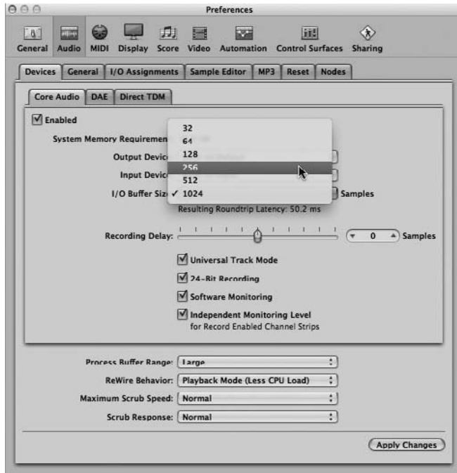
Figure 5.41 The I/O Buffer Size pop-up menu lets you choose the size of the audio buffer Logic uses when streaming digital audio into and out of Logic.
